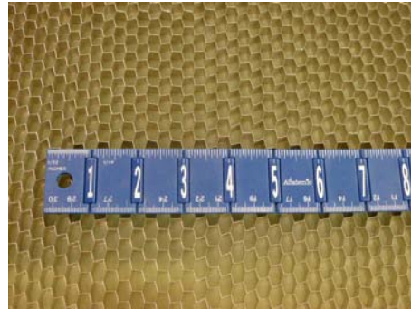
Figure 2. Honeycomb panel
