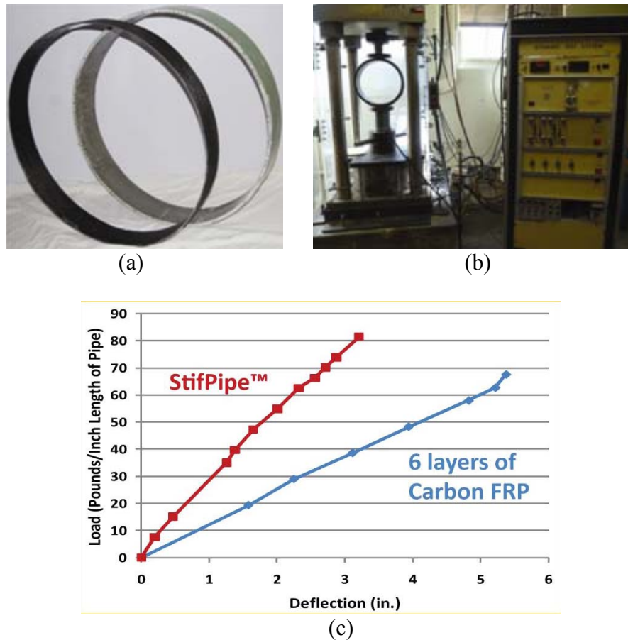
Figure 6. Comparison of 36-inch diameter carbon FRP pipe with honeycomb-FRP pipe: (a) samples; (b) test setup; (c) load vs. deflection
