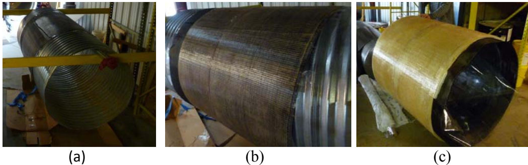
Figure 3. Steps in construction of honeycomb-FRP pipe
