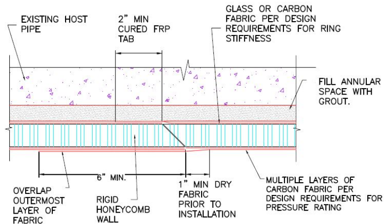
Figure 5. Connection detail at ends of honeycomb-FRP pipe.
